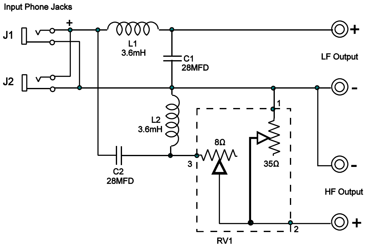
N501-8A Crossover Network (500 Hz)
